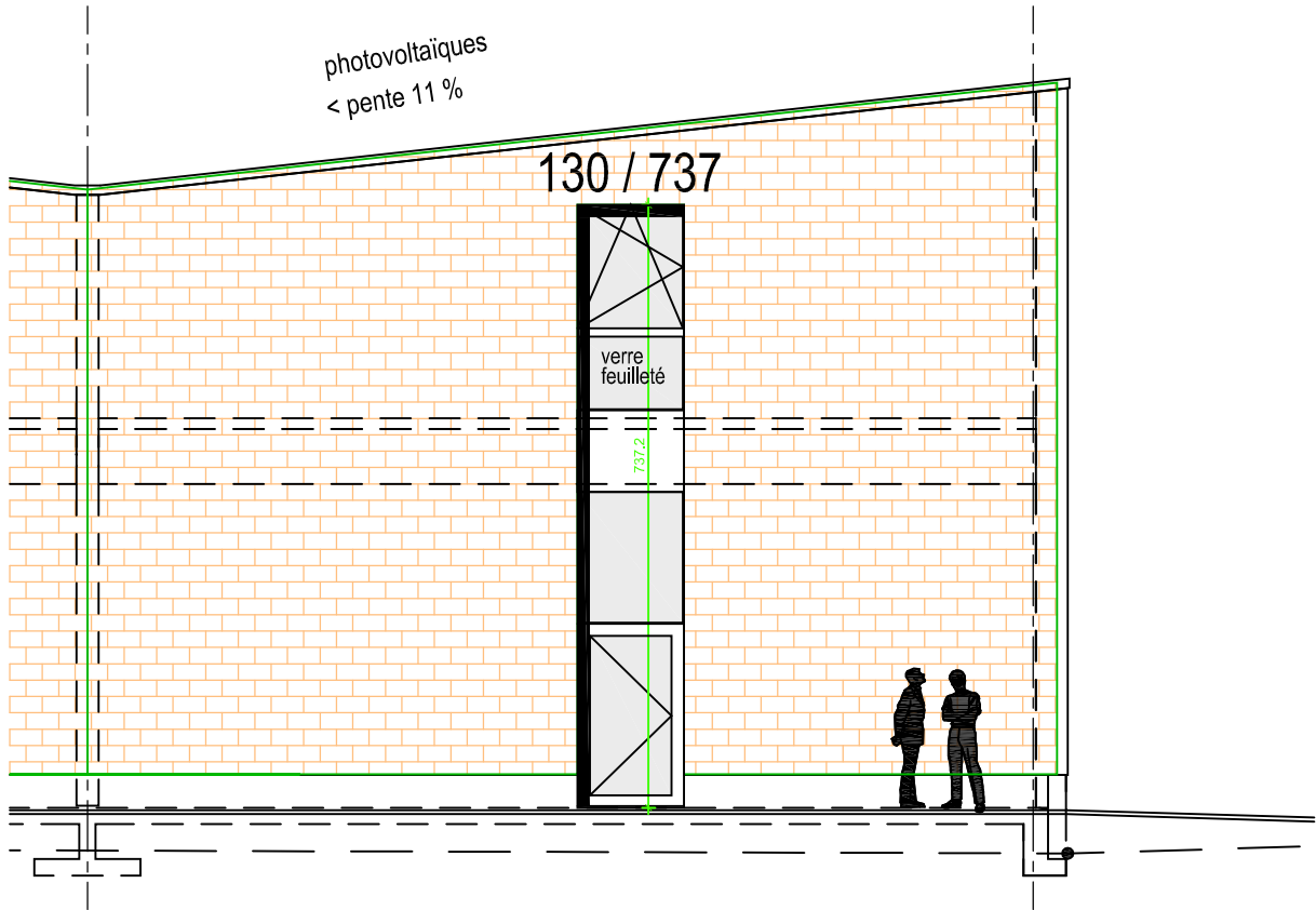
FACADE LATERALE
