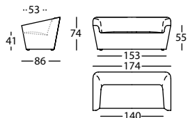
250.61.T TEA SOFA 174 TEA NON QUILTED SOFA 174 TEA CANAPE 174
