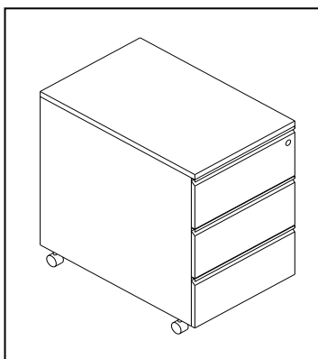
Art.54 10 110 Pedestal Three Drawers Melamine Top 46x60x57
